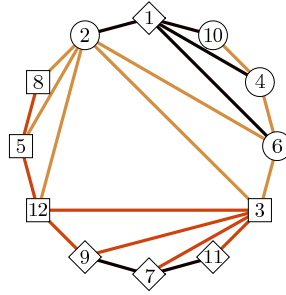
Fig. 5. Outerplanar graph G used as an example for embedding on star-shaped levels.
