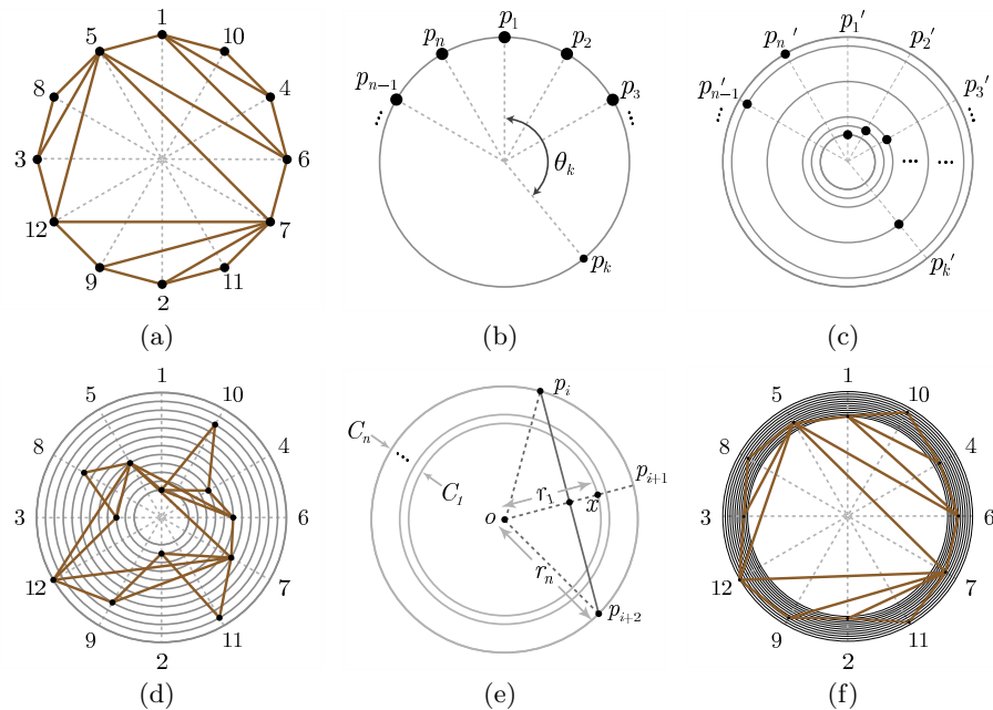
Fig. 2. The vertices of an 12-vertex outerplanar graph G are embedded on a circle in (a). This embedding follows the general point set \mathcal{P} given in (b). The points are then perturbed radially inward so that each vertex with label j lies on C_j for j = 1, 2, \dots, 12 , where C_{12} is the outermost circle in yielding point set \mathcal{P}' in (c). Drawing G on \mathcal{P}' gives (d). Crossings are then avoided by restricting the ratio between the radii of the innermost and outermost circles in (e) giving (f).
